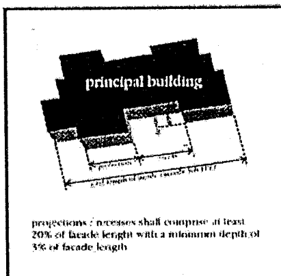
Figure 3: Example of Wall Projections and Recesses (Drawing courtesy of City of Fort Collins, Colorado Design Standards and Guidelines for Large Establishments)
