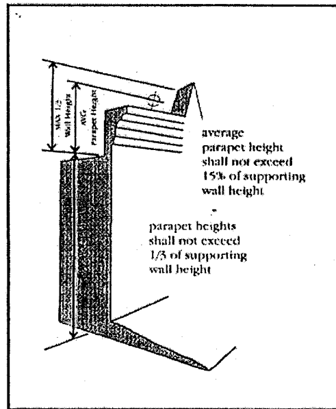
Parapet Standards.
